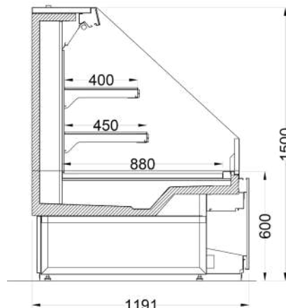
EMOTION SV 122/150
