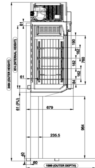
GANIMED XL TOP P&P side view
